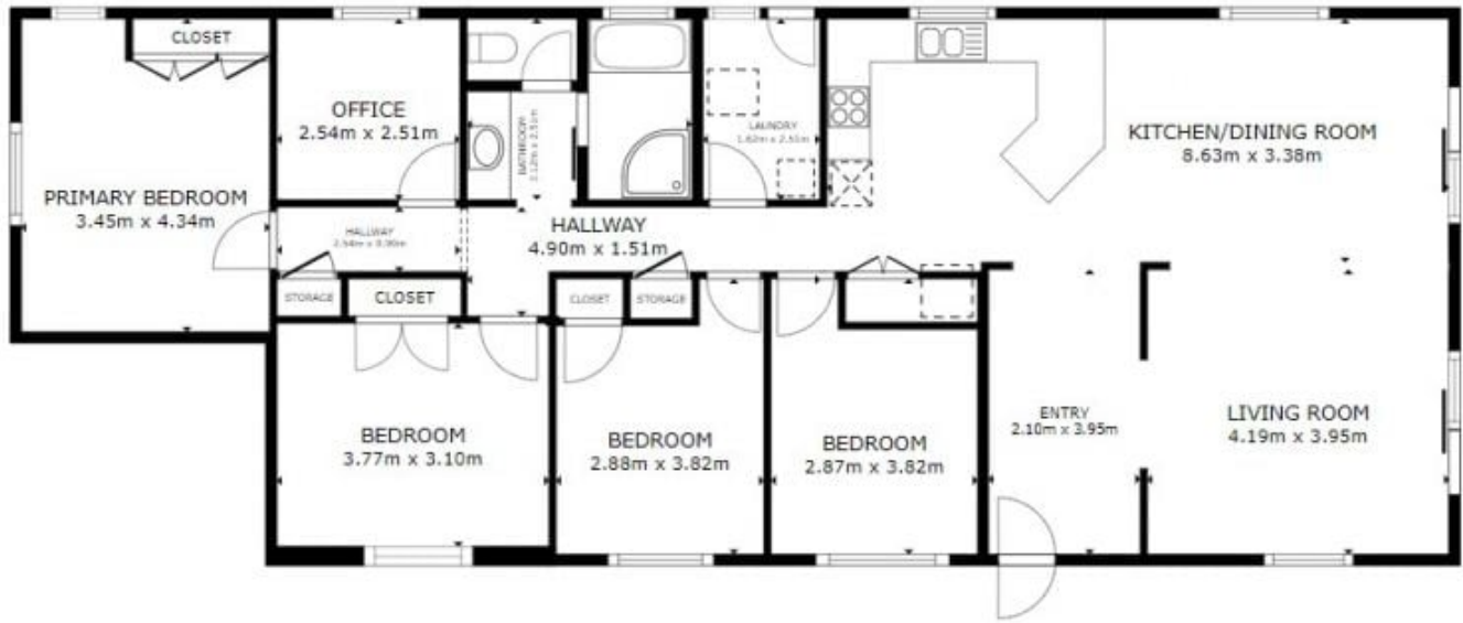
FLOOR PLAN
